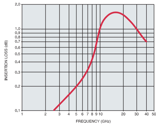
Insertion Loss of SMARTS II* Weatherproof Housing
